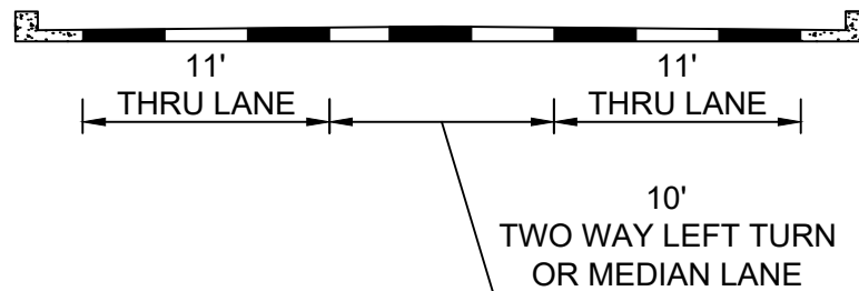
LANEAGE SECTION NOT TO SCALE
