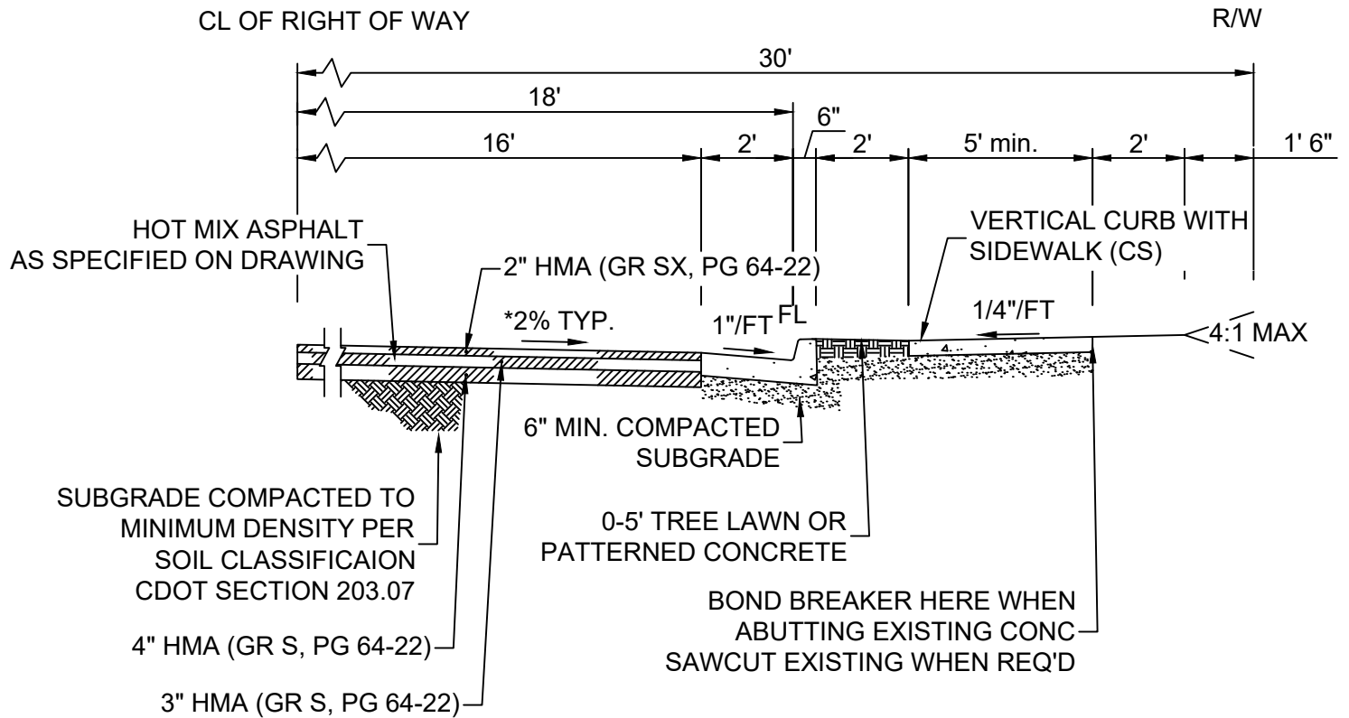
DETAIL SECTION
