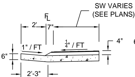
SECTION B-B MOUNTABLE CURB
