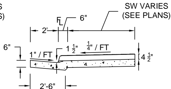
SECTION B-B VERTICAL CURB
